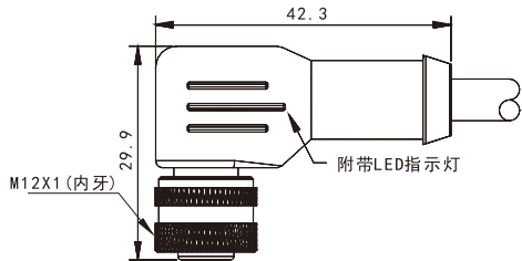
M12 母头,弯头,带LED灯,PNP
